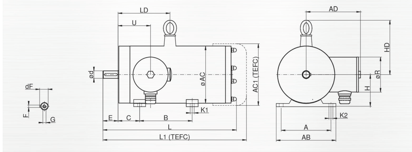
B3 DRAWING
