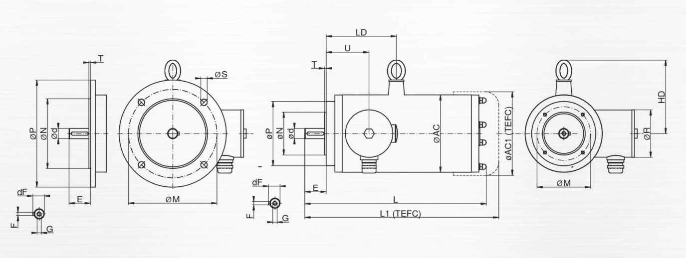
B5 / B14 DRAWING
